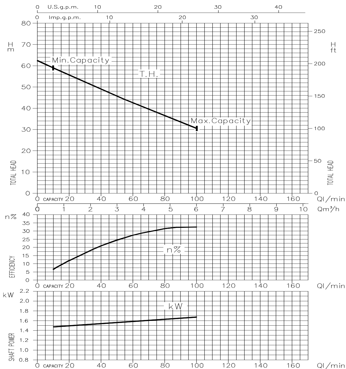
AGA 2.00 - Impeller diameter = 157 mm
