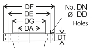
Round flange
