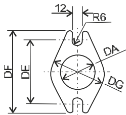
Oval flange
